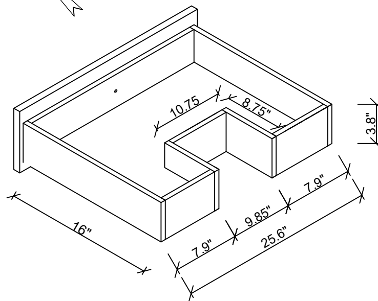
Lower drawer
