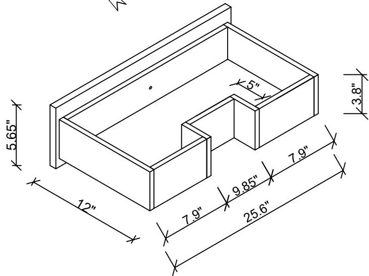
Top drawer
